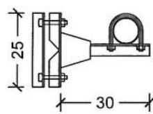
TYP 3M ANTENNA SUPPORT
